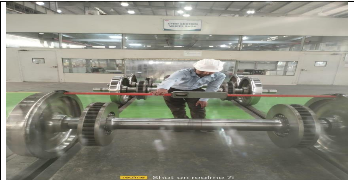
MEASUREMENT OF WHEEL GAUGE
